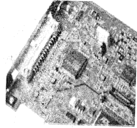
Assembled PCB
